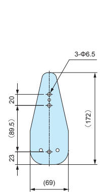
Wall mounting bracket dimensions
