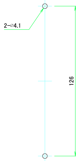
*取付穴寸法 / Mounting hole dimensions
