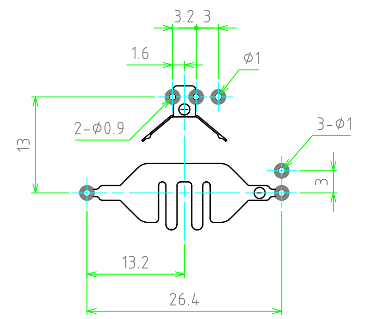
シルク印刷部詳細 Battery contact position details
