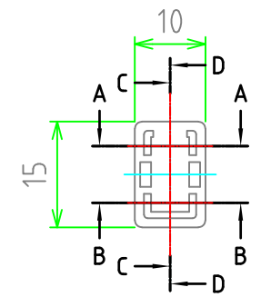
下蓋 (内視) Cover (Internal View)
