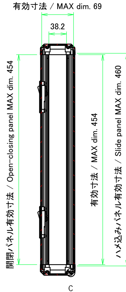
B-B (1:5)
