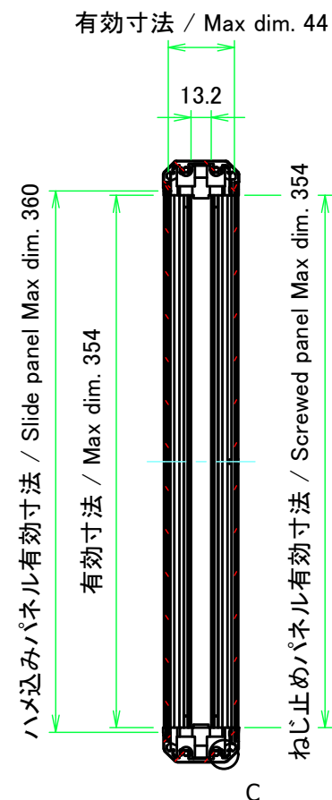
B-B (1:4.5)
