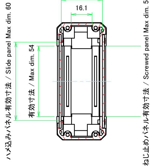
B-B (1:1.5)
