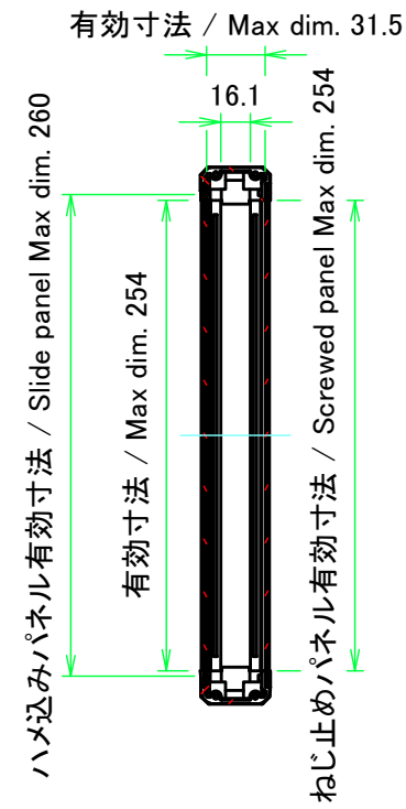
B-B (1:4.5)
