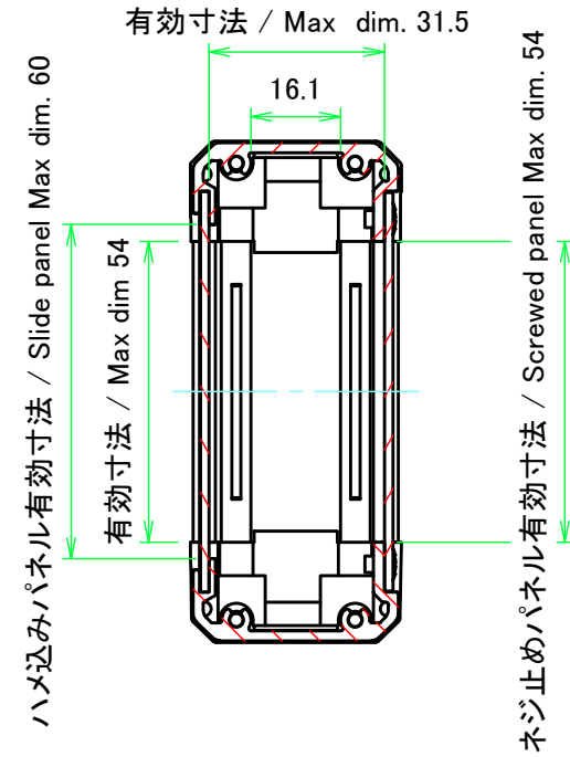
B-B (1:1.5)
