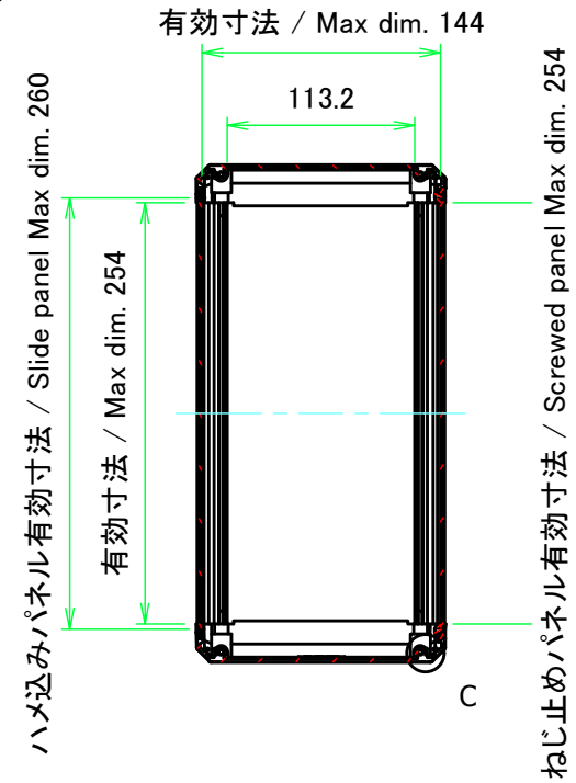
B-B (1:5)
