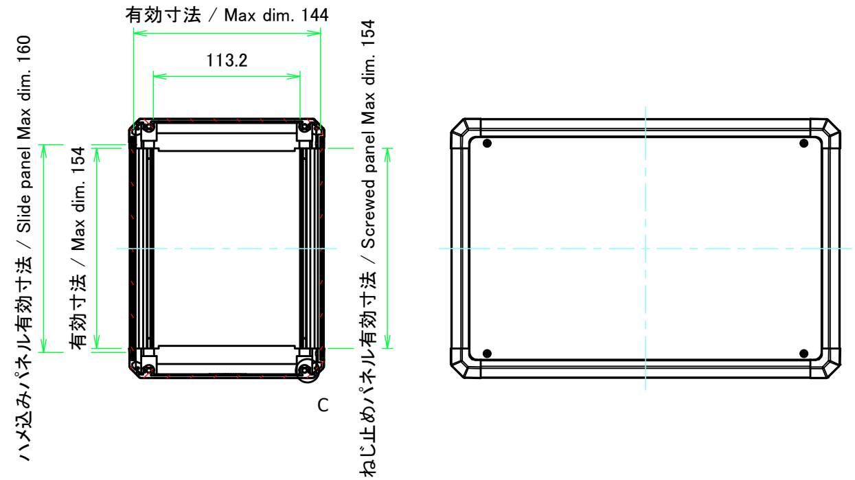
B-B (1:4)
