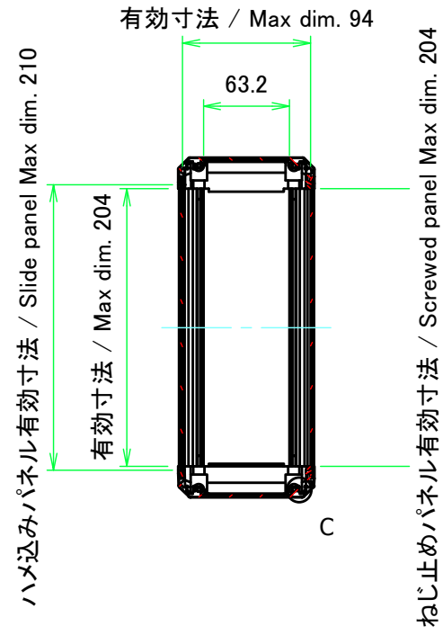
B-B (1:5)
