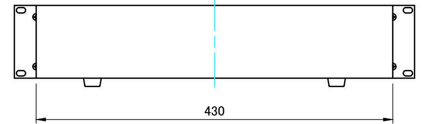
B view
