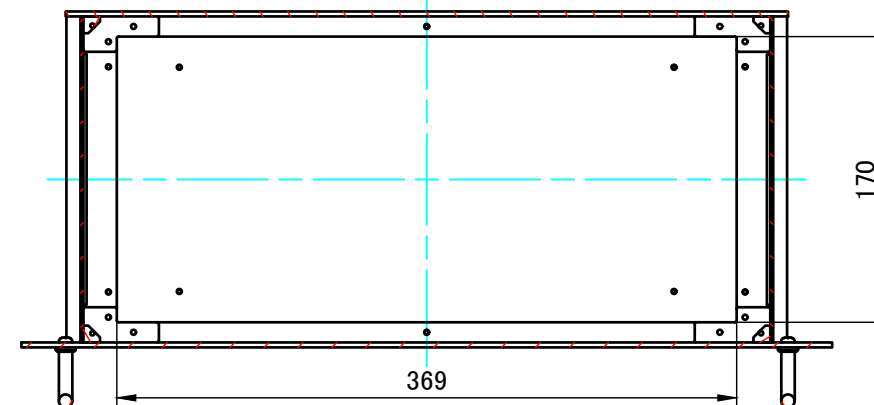
B-B (1:4.5)
