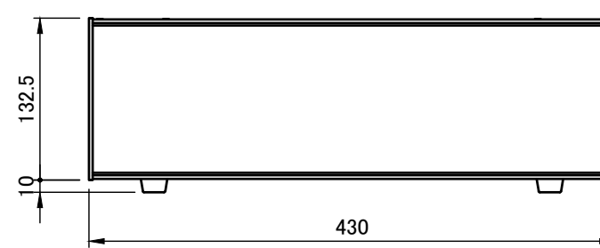
B-B (1:5.5)
