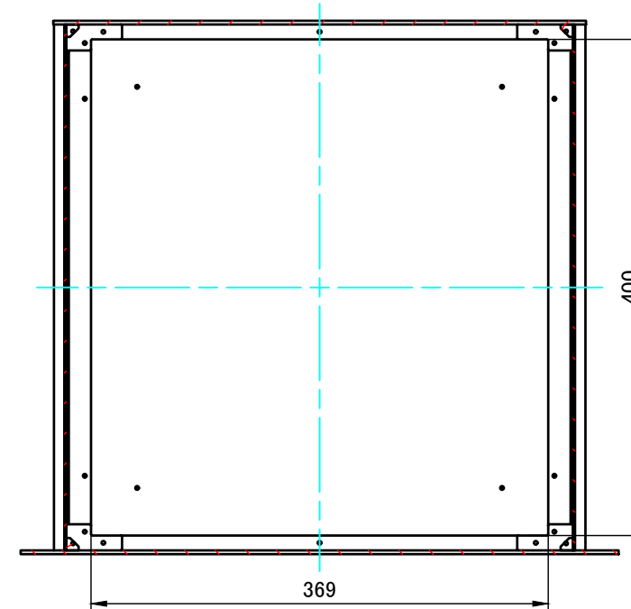
B-B (1:5.5)
