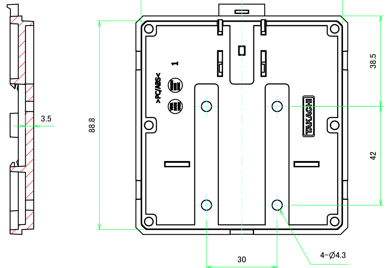
B-B (1:1)
