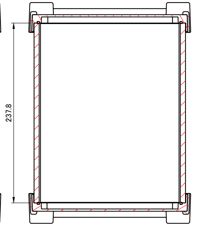
C-C (1:3)
